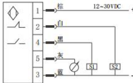
2 X NPN + analog output
